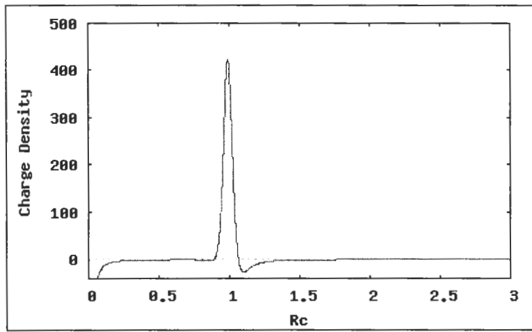
Fig. 5a-d. Generalized Kerr-Newman, q=1 , a=2 , \alpha=1 , \theta=\pi/2
