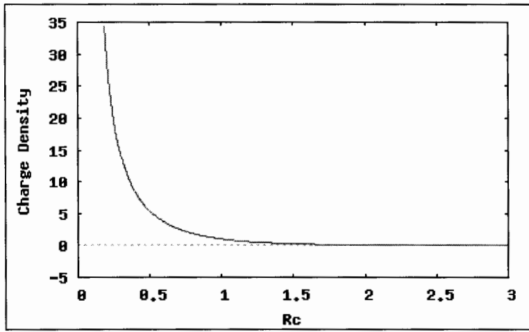
Fig. 4a-d. Generalized Kerr-Newman, q=1 , a=0 , \alpha=1 , \theta=\pi/2
