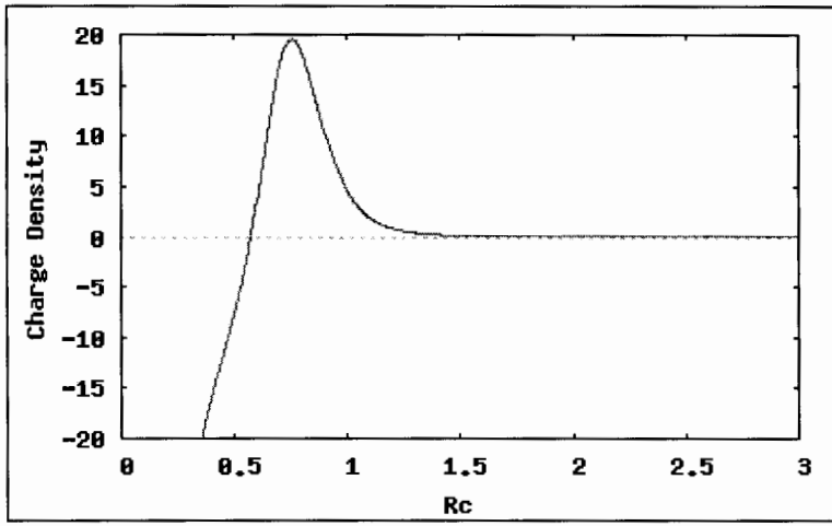
Fig. 2a-d. Generalized Kerr-Newman, q=1 , a=1 , \alpha=1 , \theta=\pi/2
