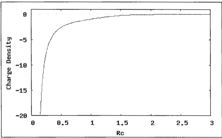
Fig. 3a-d. Generalized Kerr-Newman, q=0 , a=1 , \alpha=1 , \theta=\pi/2
